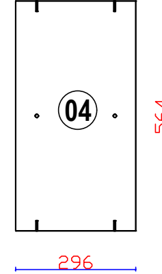
SABİT RAF
